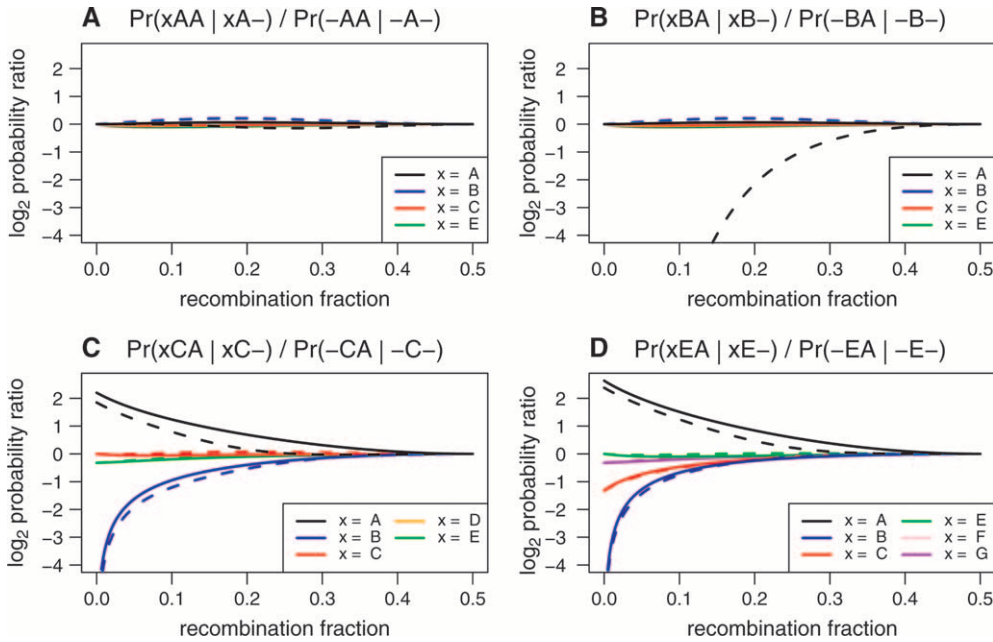
FIGURE 5.—Assessment of the Markov property in the three-point probabilities on autosomes of eight-way RILs by sibling mating. \text{Log}_2\{\text{Pr}(xyA|xy-)/\text{Pr}(-yA|-y-)\} is displayed for each distinct case of x, y , with the solid and dashed curves corresponding to no interference and strong positive crossover interference, respectively.
