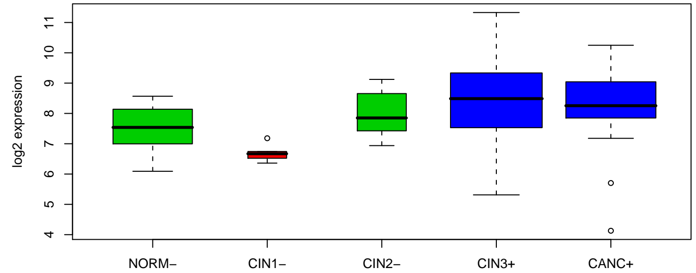
HIST1H2BD (222067_x_at)
