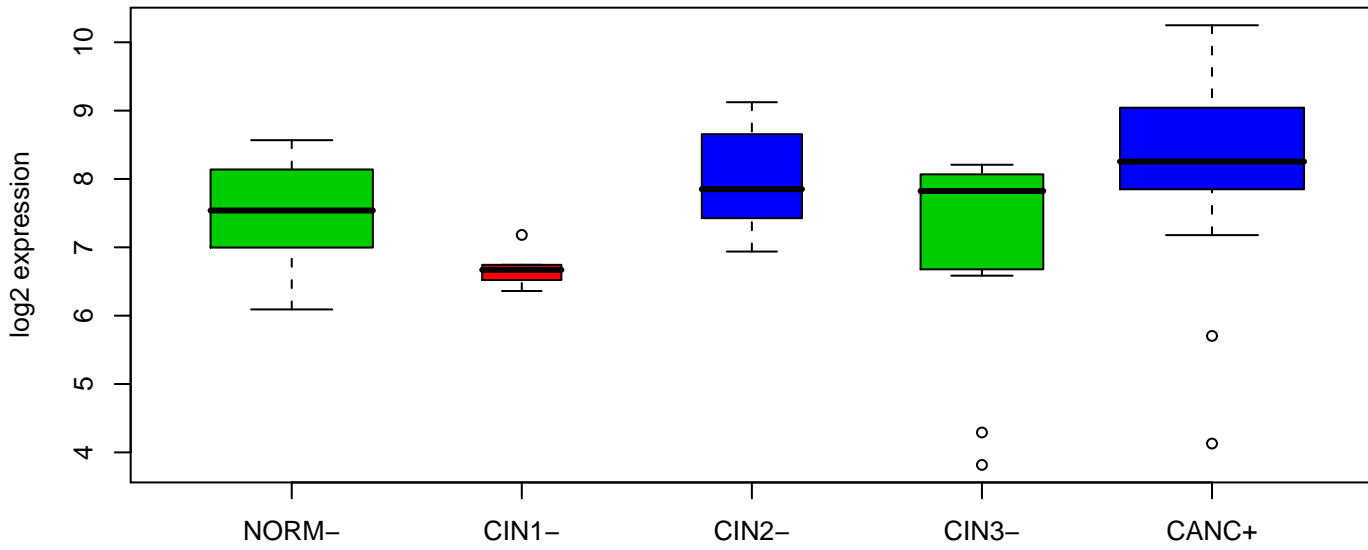
HIST1H2BD (222067_x_at)
